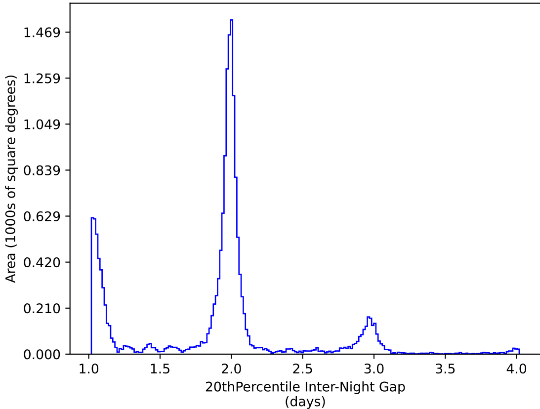
weather_cloudso14v3.4_10yrs WFD y band: 20thPercentile Inter-Night Gap
