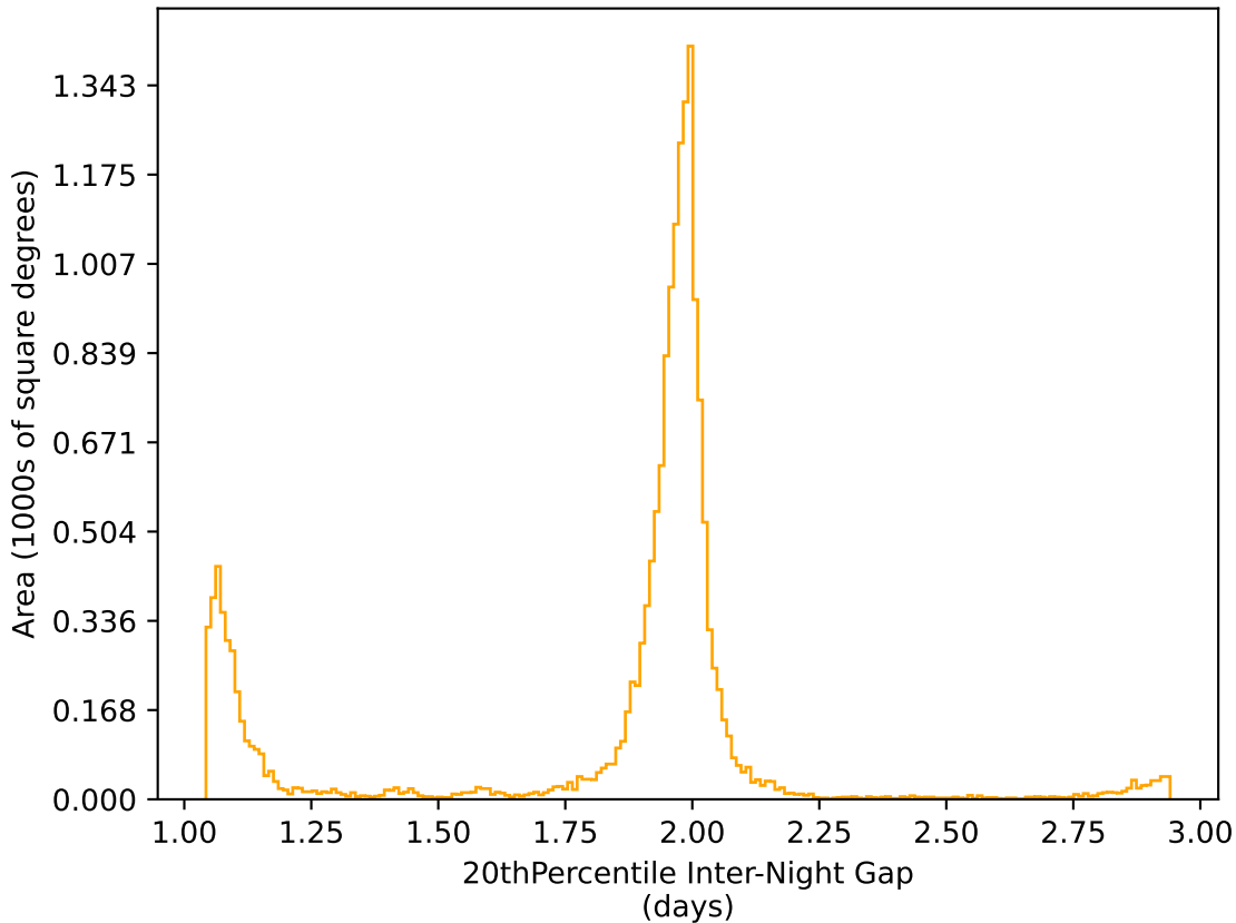
weather_cloudso14v3.4_10yrs WFD r band: 20thPercentile Inter-Night Gap
