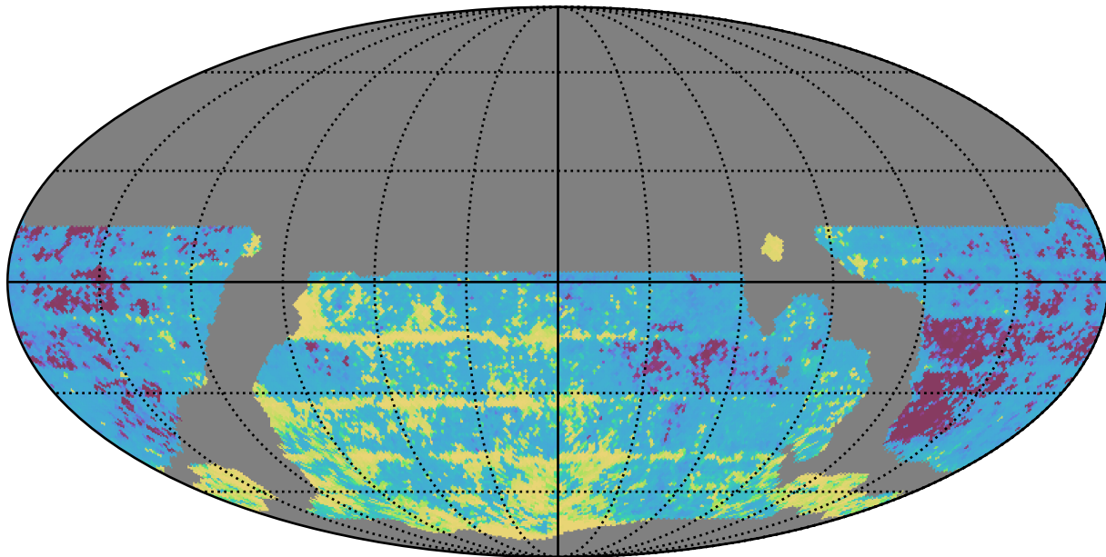
weather_cloudso14v3.4_10yrs WFD i band: 20thPercentile Inter-Night Gap
