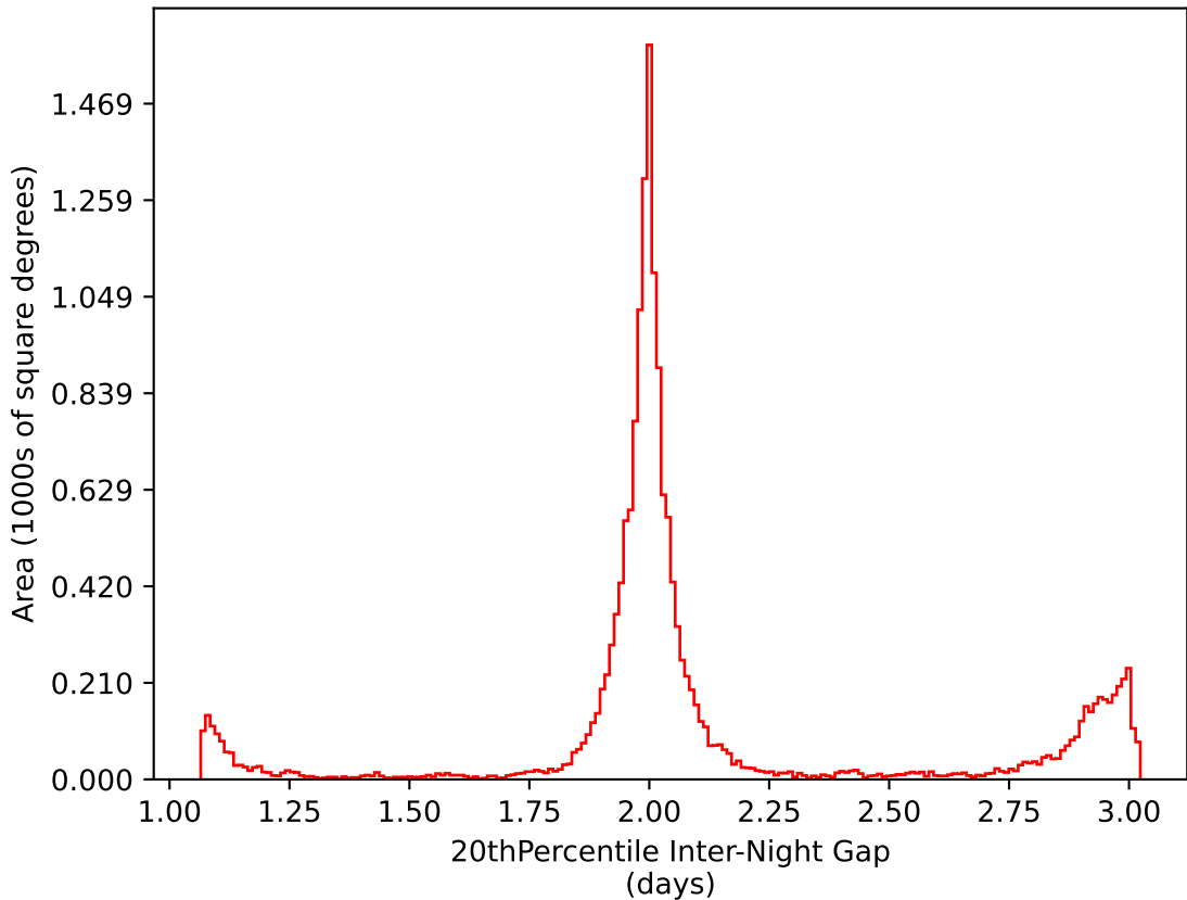
weather_cloudso14v3.4_10yrs WFD i band: 20thPercentile Inter-Night Gap
