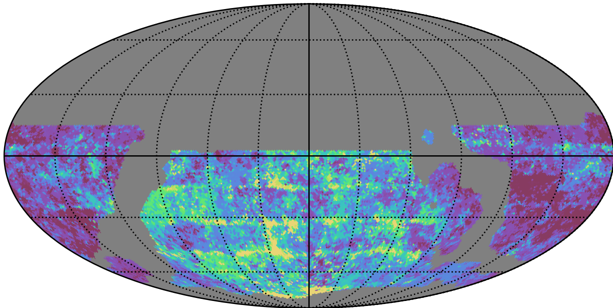
weather_cloudso14v3.4_10yrs WFD g band: 20thPercentile Inter-Night Gap
