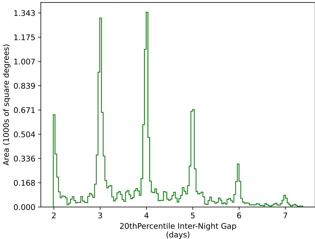
weather_cloudso14v3.4_10yrs WFD g band: 20thPercentile Inter-Night Gap
