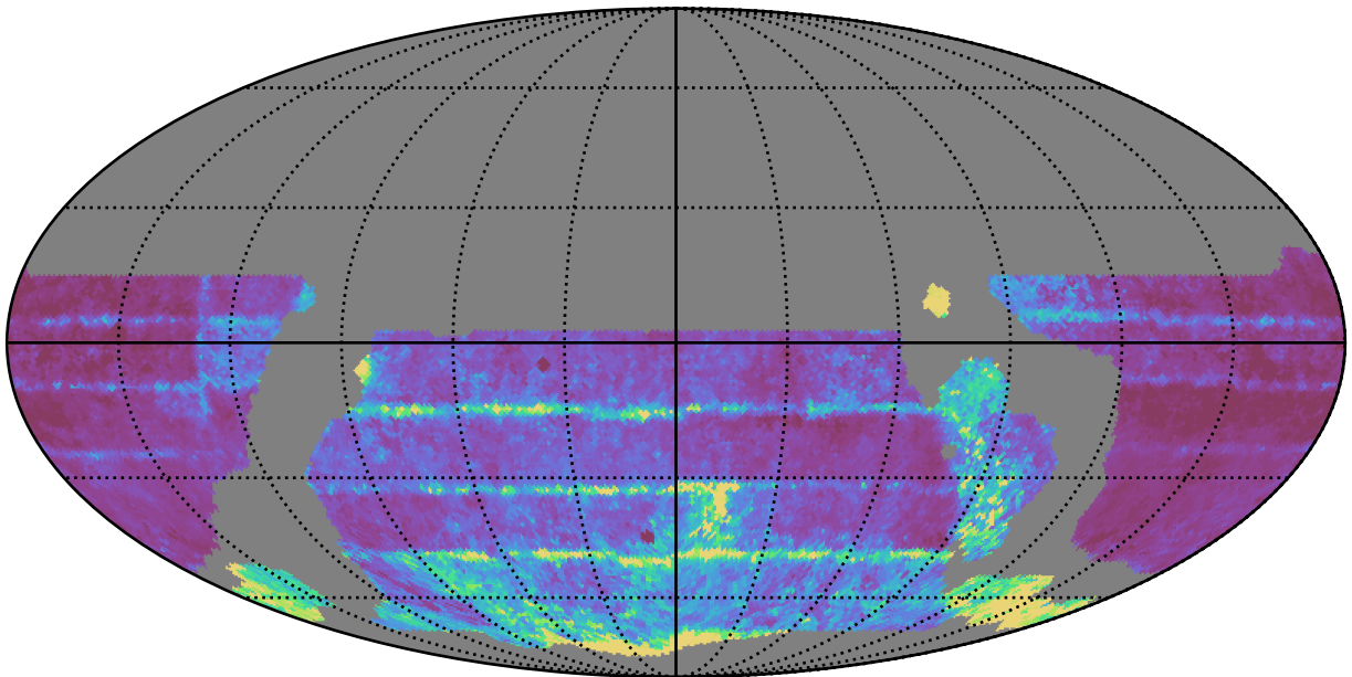
weather_cloudso14v3.4_10yrs WFD all bands: 20thPercentile Inter-Night Gap
