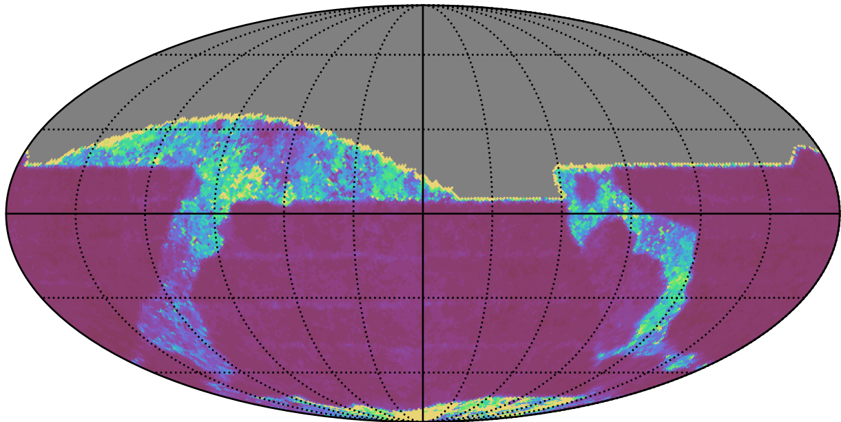
weather_cloudso14v3.4_10yrs All sky z band: 20thPercentile Inter-Night Gap
