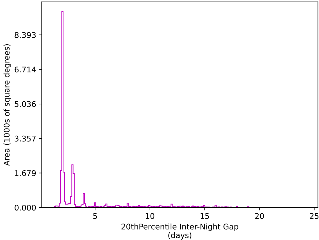
weather_cloudso14v3.4_10yrs All sky z band: 20thPercentile Inter-Night Gap
