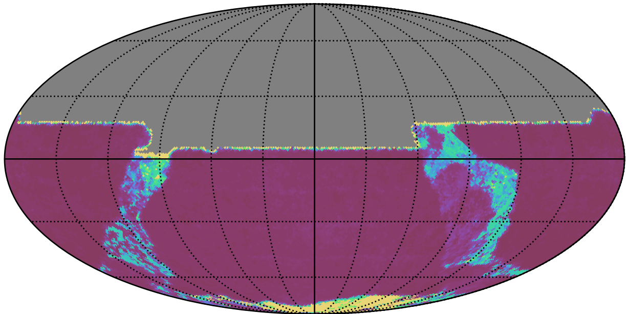
weather_cloudso14v3.4_10yrs All sky y band: 20thPercentile Inter-Night Gap
