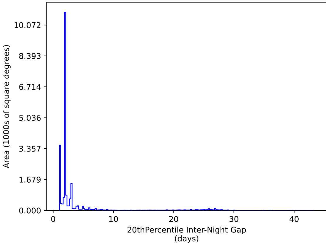
weather_cloudso14v3.4_10yrs All sky y band: 20thPercentile Inter-Night Gap
