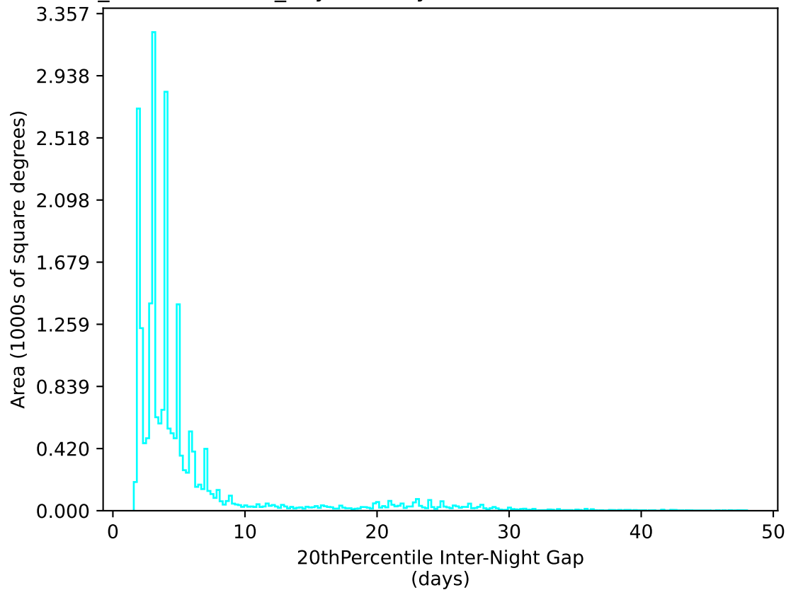
weather_cloudso14v3.4_10yrs All sky u band: 20thPercentile Inter-Night Gap
