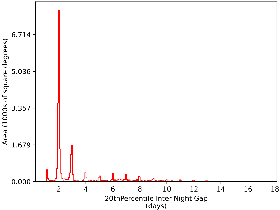
weather_cloudso14v3.4_10yrs All sky i band: 20thPercentile Inter-Night Gap
