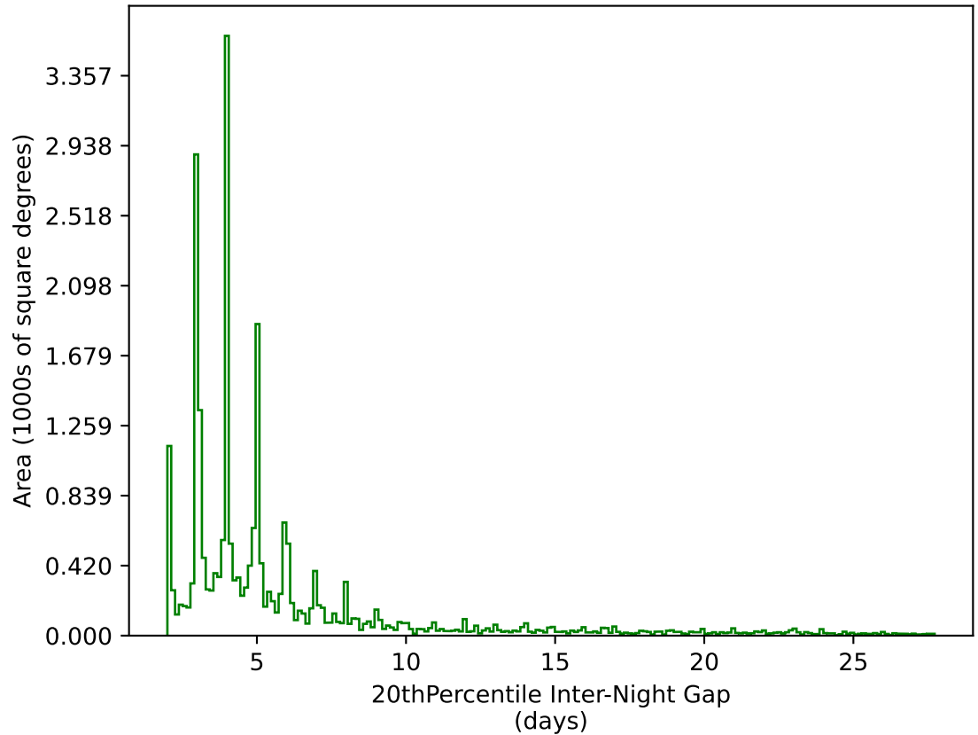
weather_cloudso14v3.4_10yrs All sky g band: 20thPercentile Inter-Night Gap
