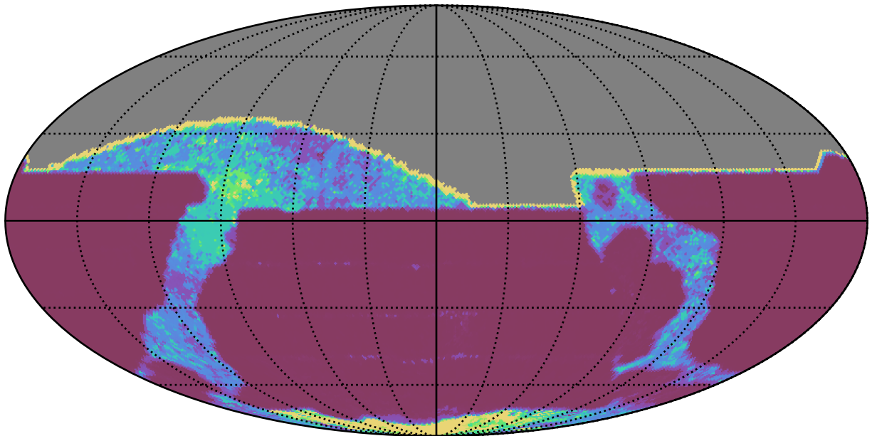
weather_cloudso14v3.4_10yrs All sky all bands: 20thPercentile Inter-Night Gap
