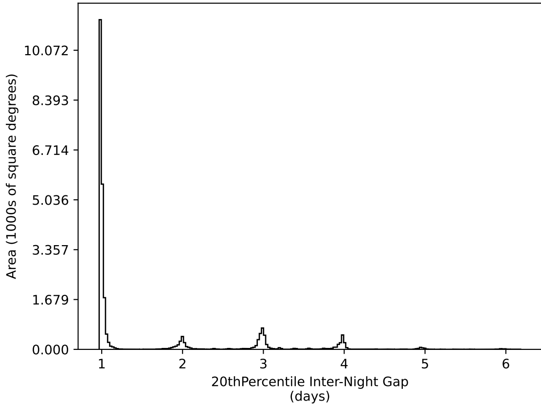
weather_cloudso14v3.4_10yrs All sky all bands: 20thPercentile Inter-Night Gap
