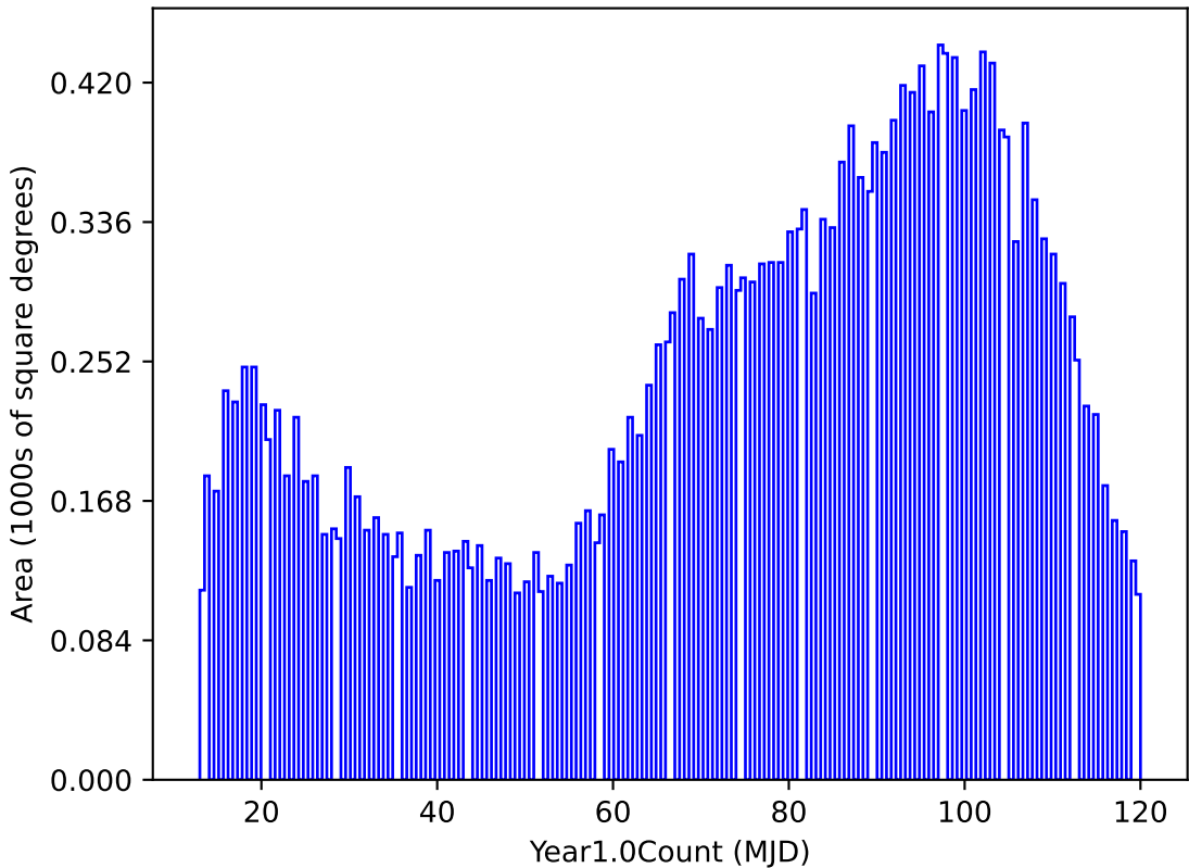
weather_cloudso14v3.4_10yrs night < 365.25: Year1.0Count
