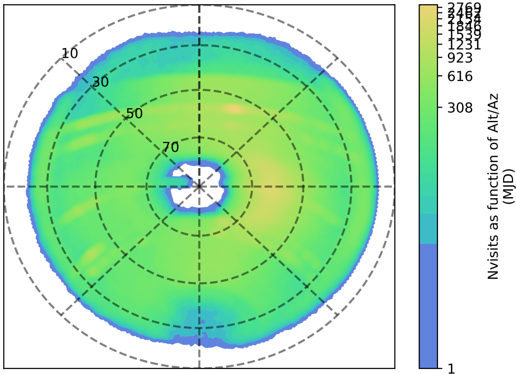
weather_cloudso14v3.4_10yrs z: Nvisits as function of Alt/Az
