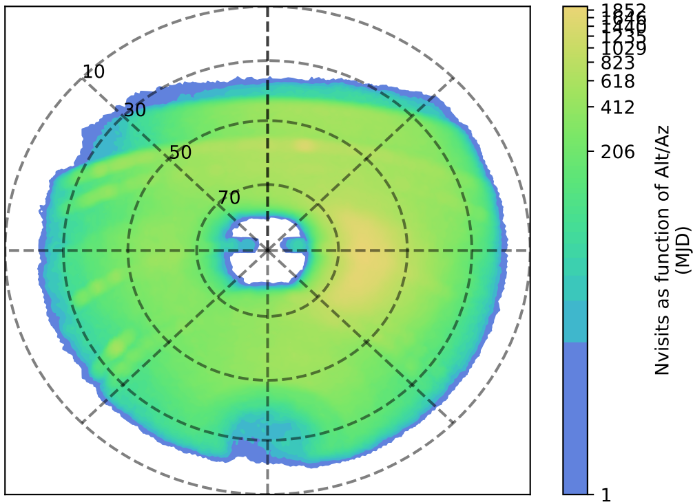
weather_cloudso14v3.4_10yrs y: Nvisits as function of Alt/Az
