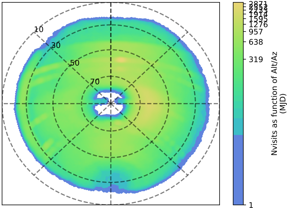
weather_cloudso14v3.4_10yrs r: Nvisits as function of Alt/Az
