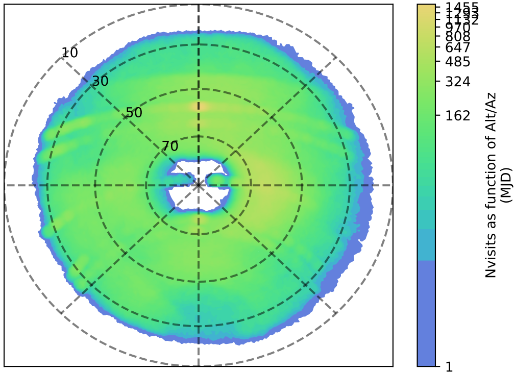
weather_cloudso14v3.4_10yrs g: Nvisits as function of Alt/Az
