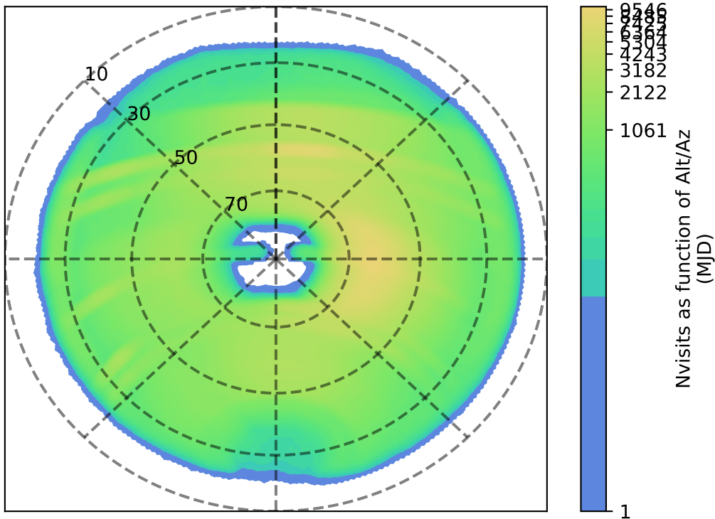
weather_cloudso14v3.4_10yrs : Nvisits as function of Alt/Az
