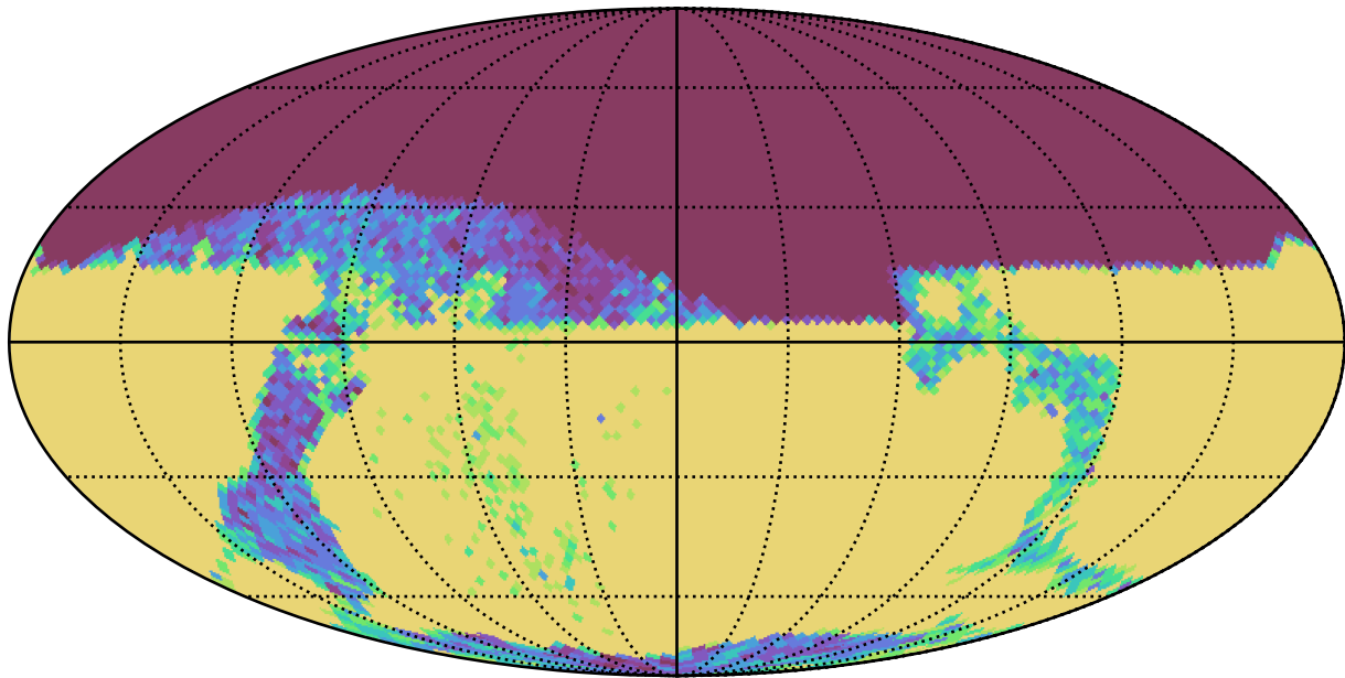
weather_cloudso14v3.4_10yrs z and night < 365: N year 1
