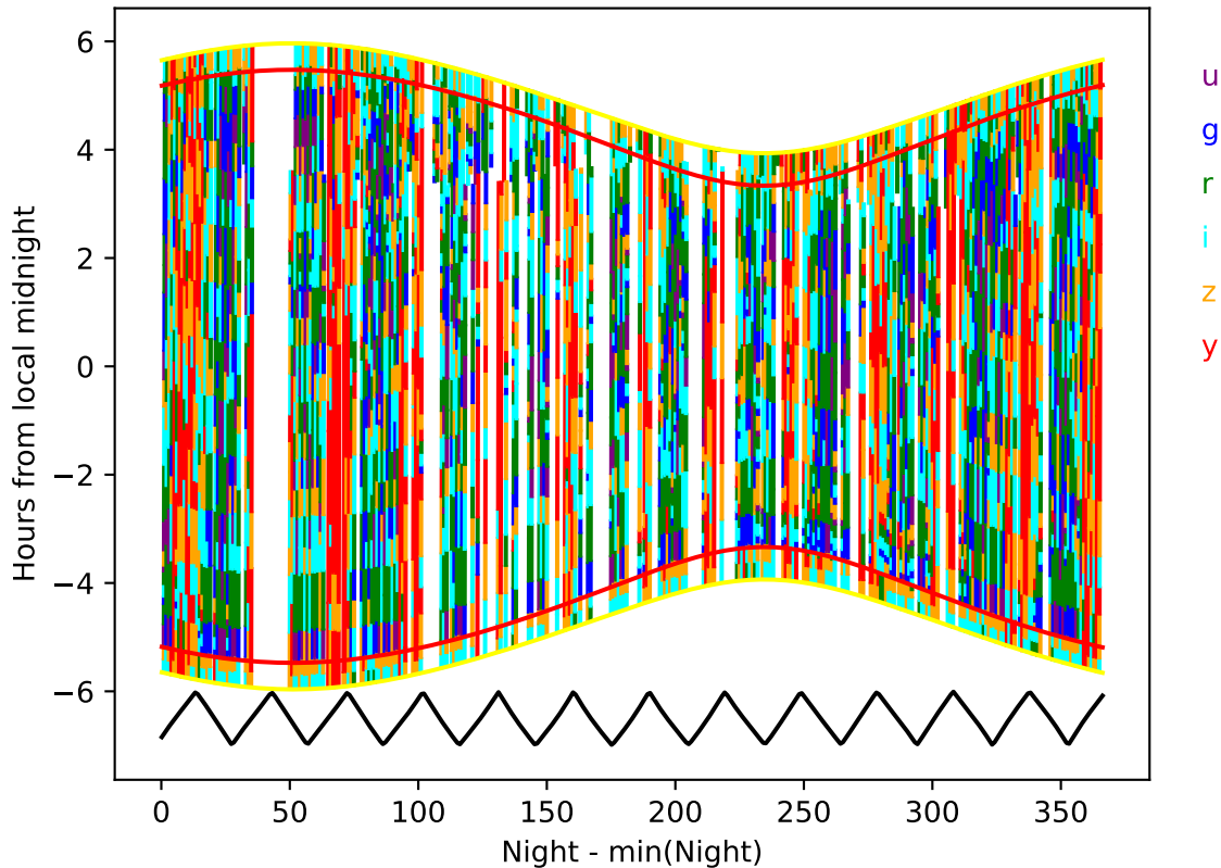
weather_cloudso14v3.4_10yrs year 8-9: Hourglass
