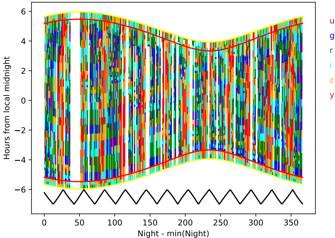
weather_cloudso14v3.4_10yrs year 4-5: Hourglass
