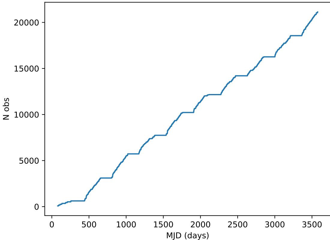
weather_cloudso14v3.4_10yrs note like DD:XMM_LSS%: Cumulative
