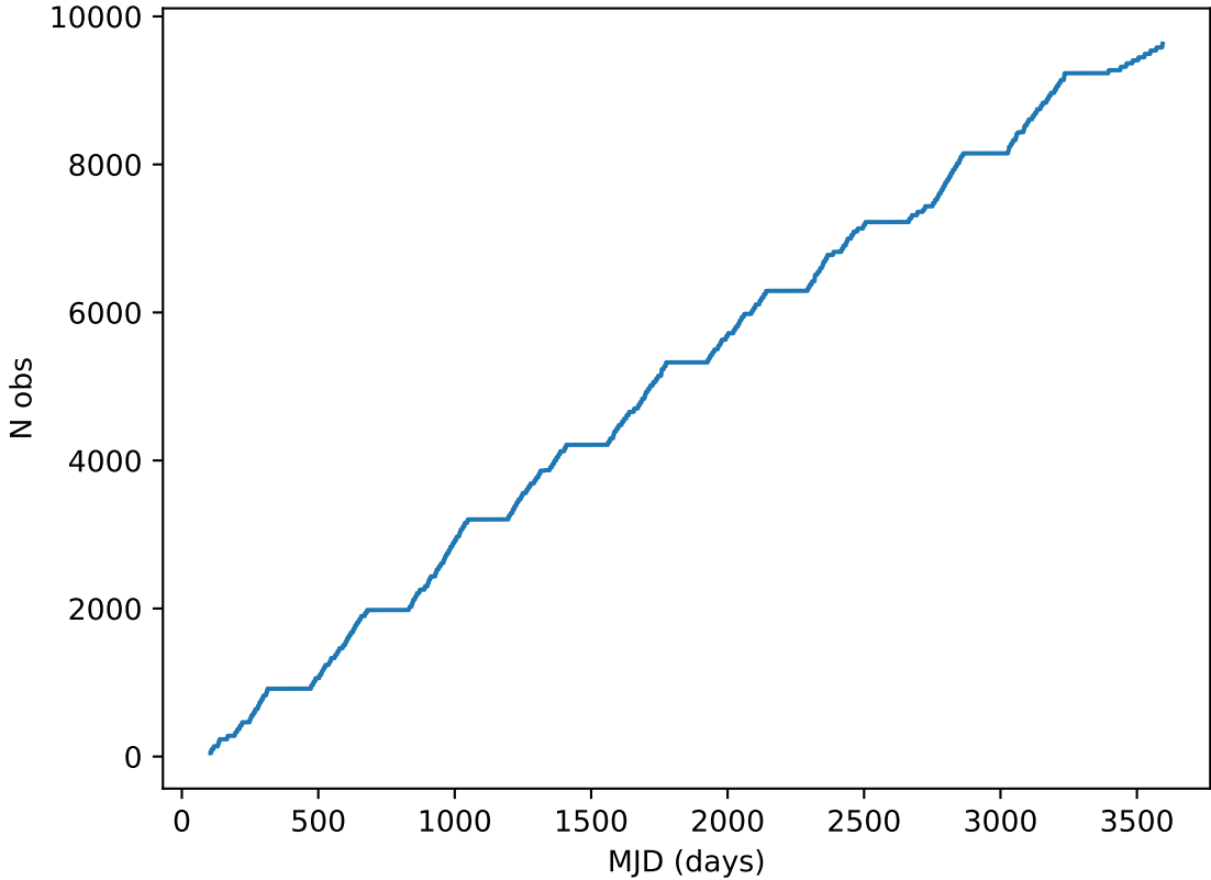
weather_cloudso14v3.4_10yrs note like DD:EDFS_b%: Cumulative
