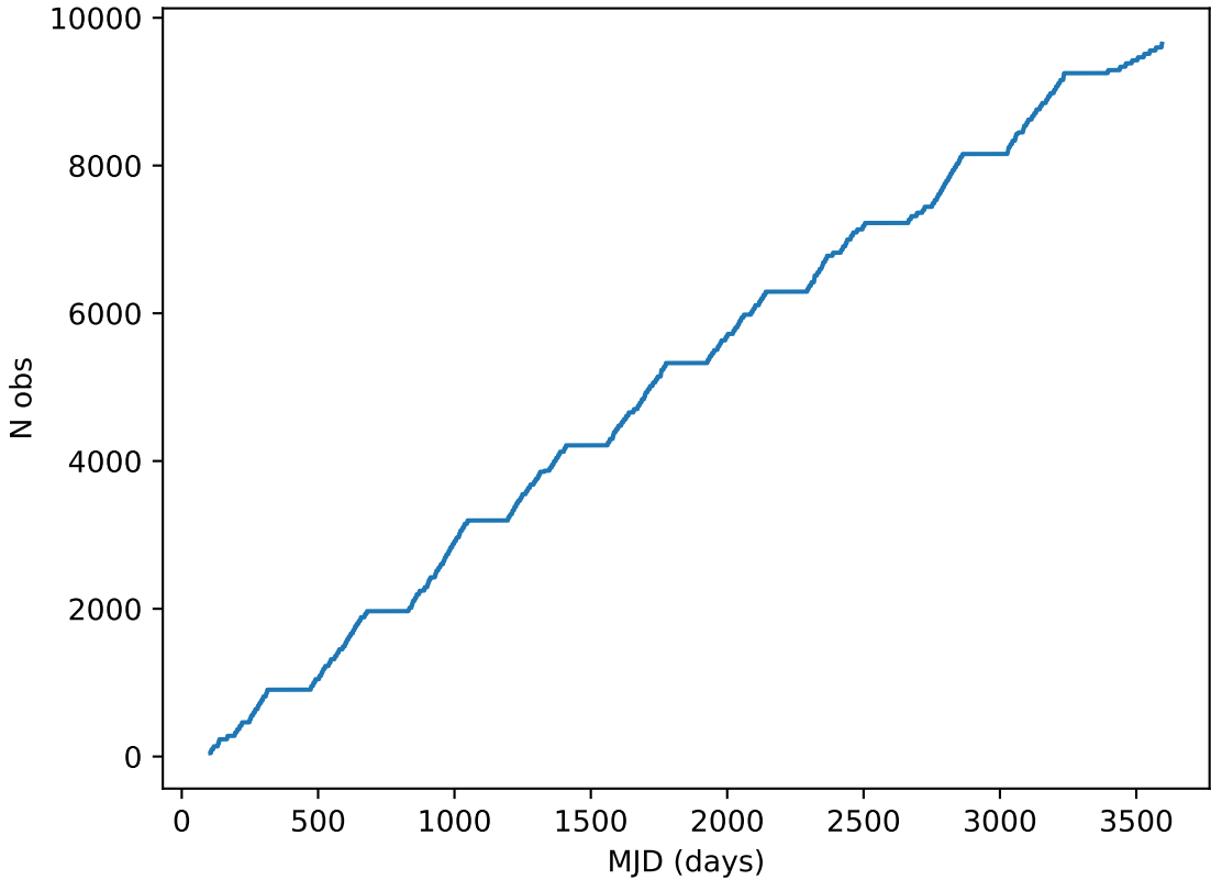
weather_cloudso14v3.4_10yrs note like DD:EDFS_a%: Cumulative
