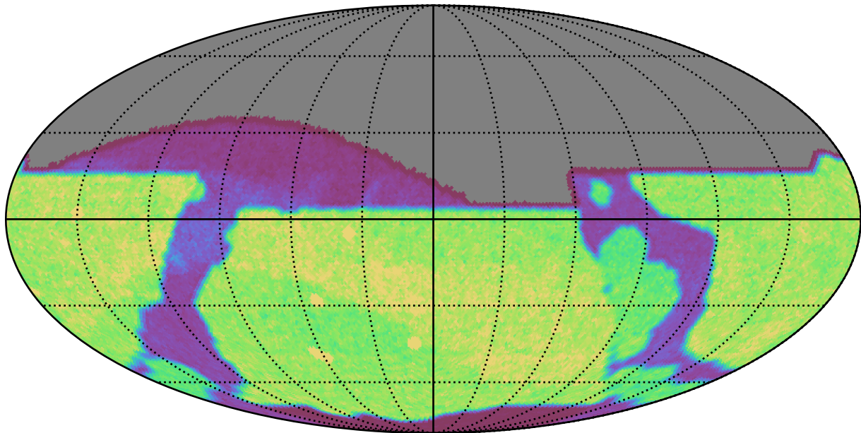
weather_cloudso14v3.4_10yrs z: Count observationStartMJD
