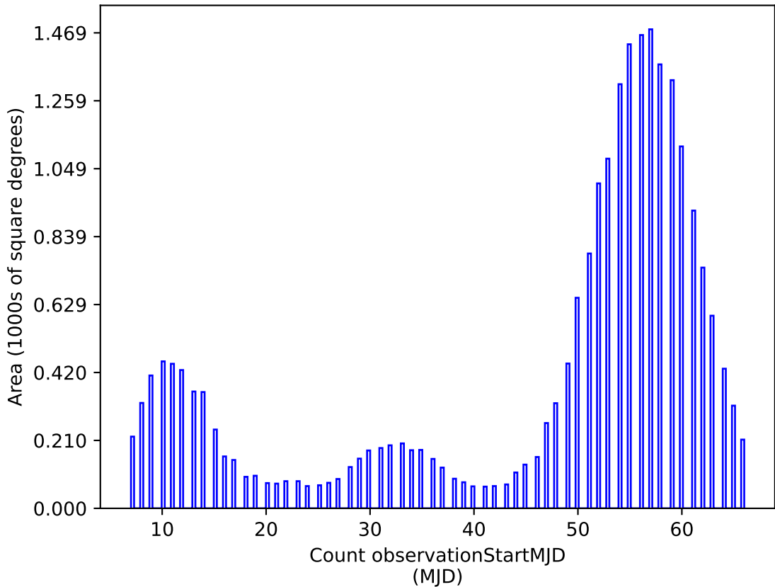
weather_cloudso14v3.4_10yrs u: Count observationStartMJD
