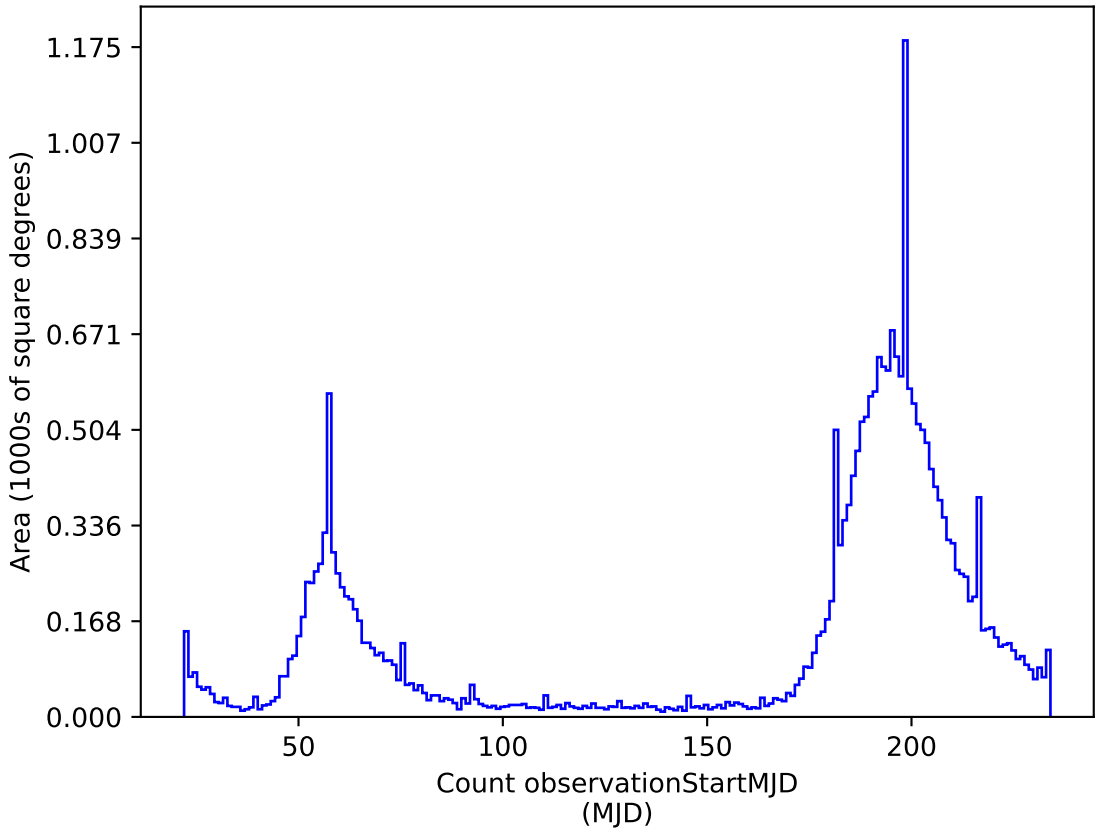
weather_cloudso14v3.4_10yrs r: Count observationStartMJD
