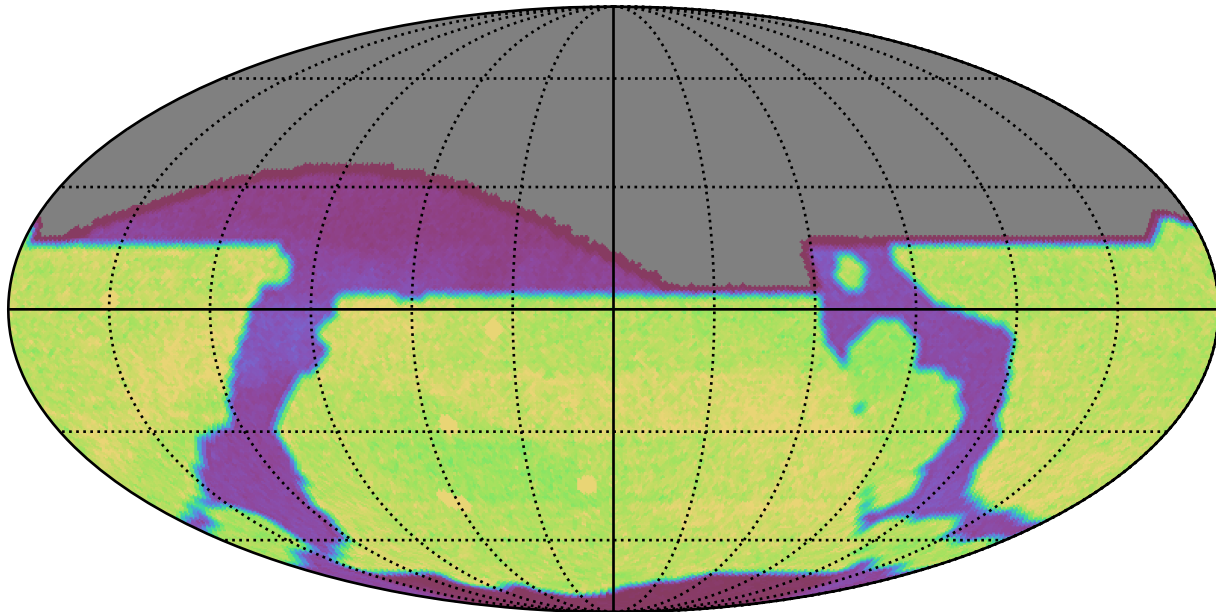
weather_cloudso14v3.4_10yrs : Count observationStartMJD
