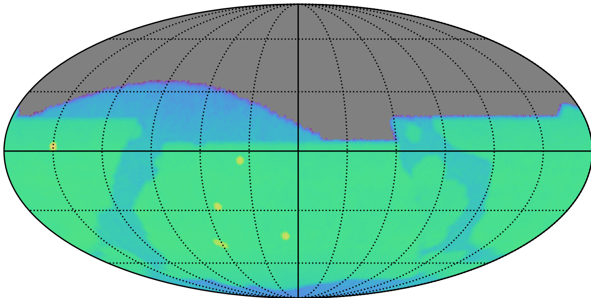
weather_cloudso14v3.4_10yrs z: CoaddM5
