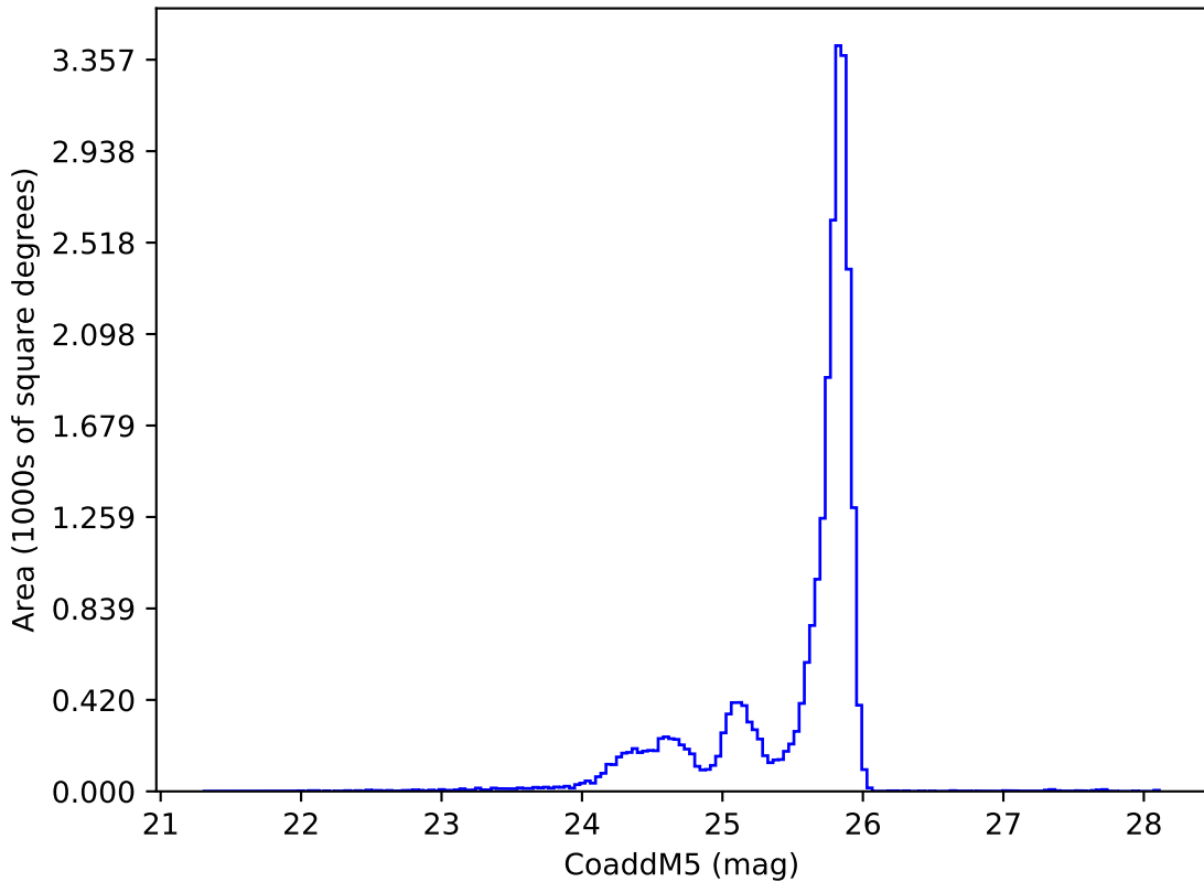
weather_cloudso14v3.4_10yrs z: CoaddM5
