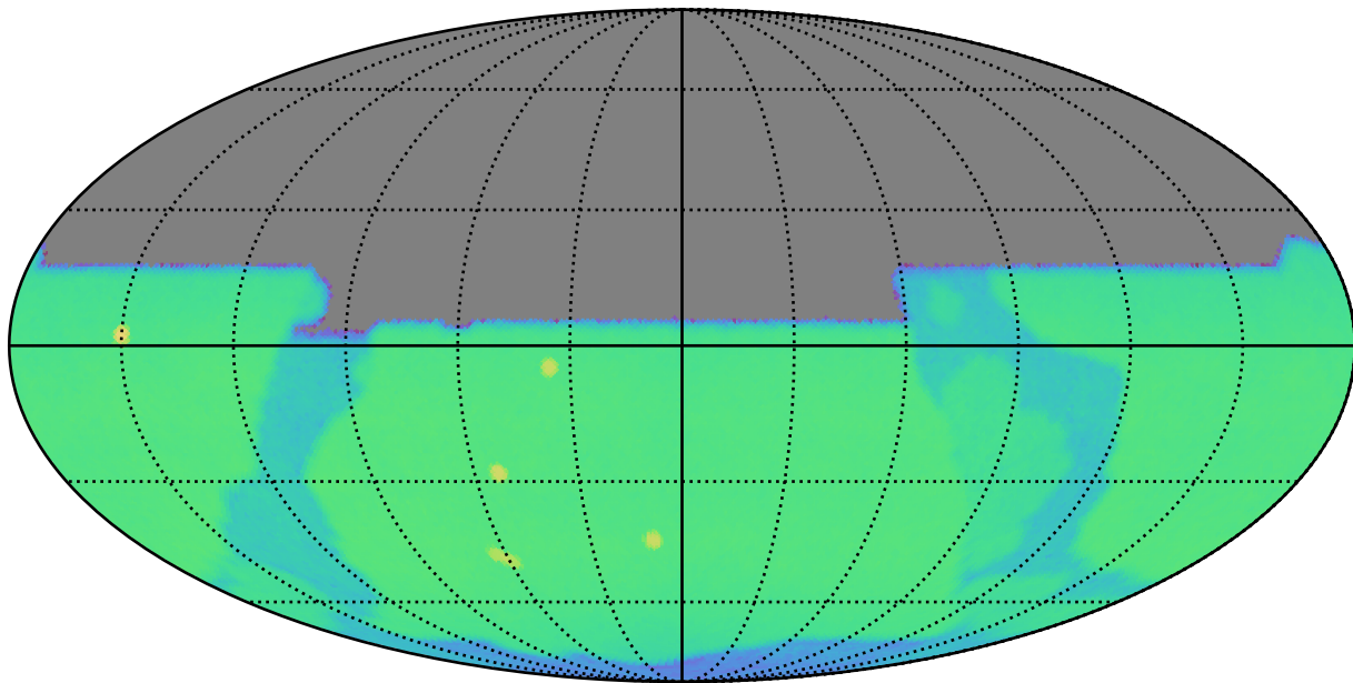
weather_cloudso14v3.4_10yrs y: CoaddM5
