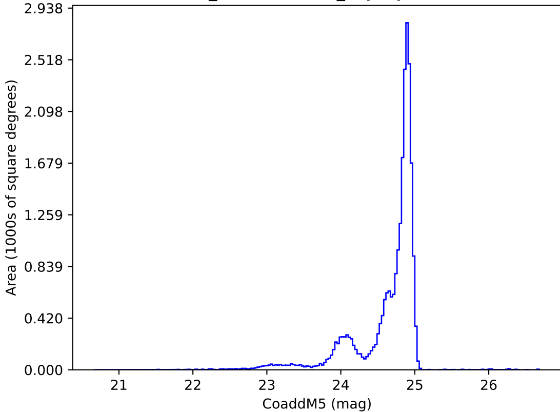
weather_cloudso14v3.4_10yrs y: CoaddM5
