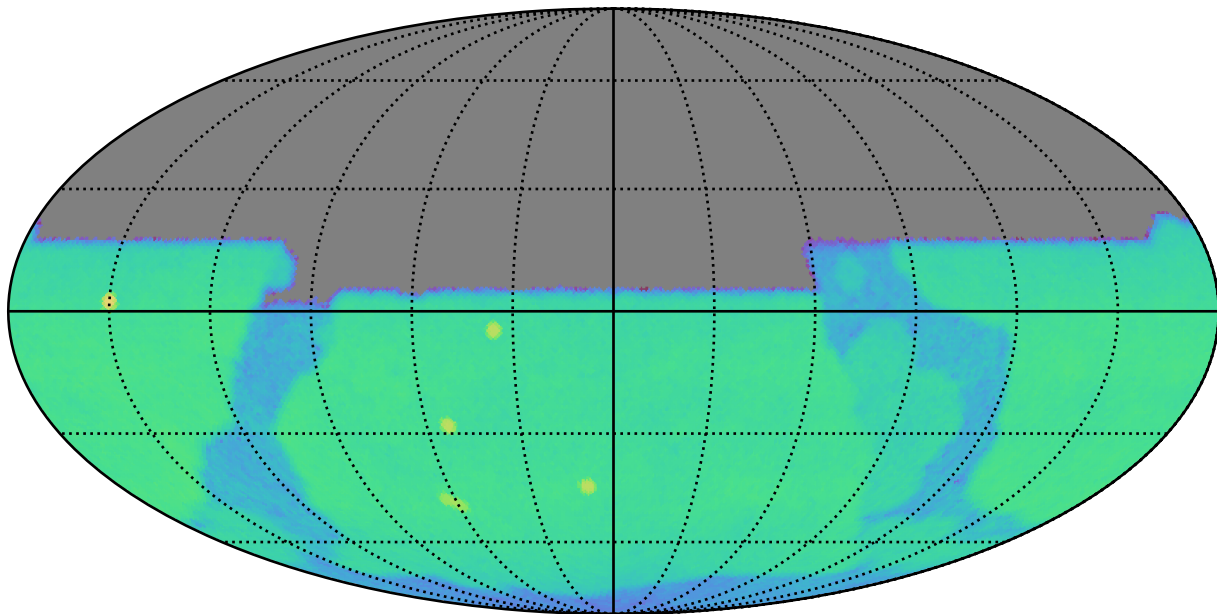
weather_cloudso14v3.4_10yrs u: CoaddM5
