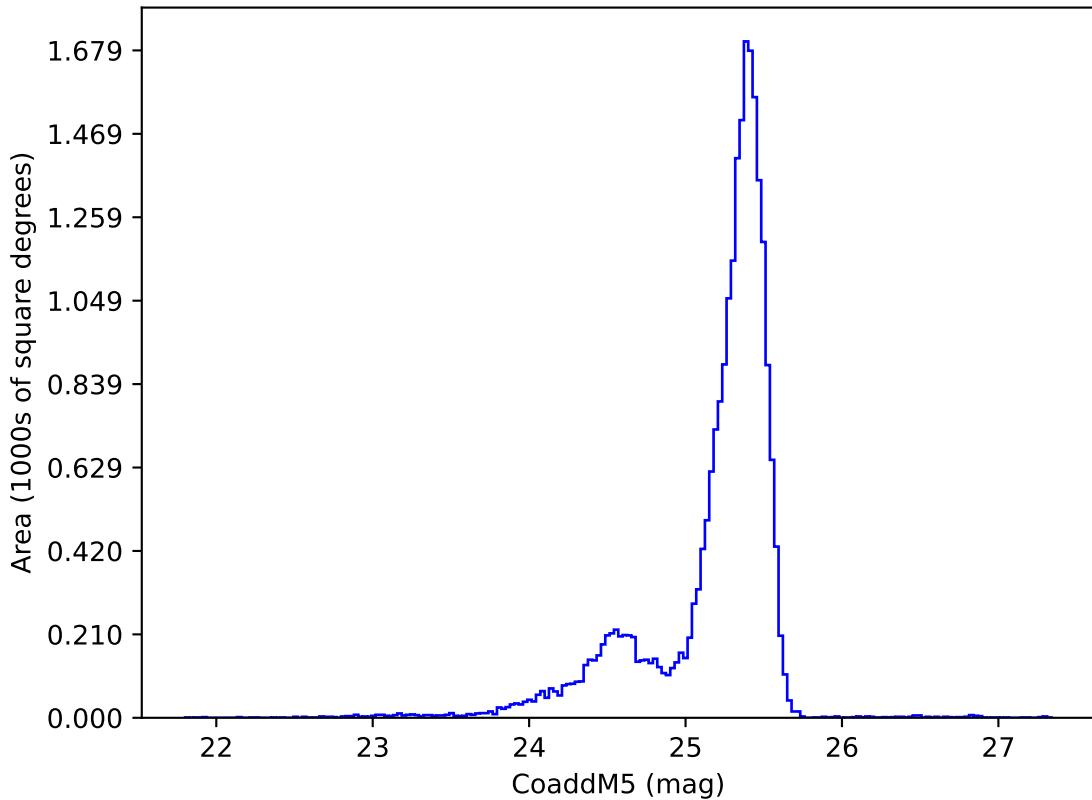
weather_cloudso14v3.4_10yrs u: CoaddM5
