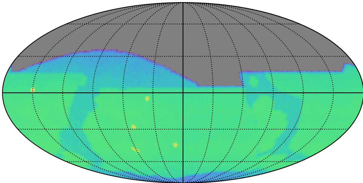
weather_cloudso14v3.4_10yrs r: CoaddM5
