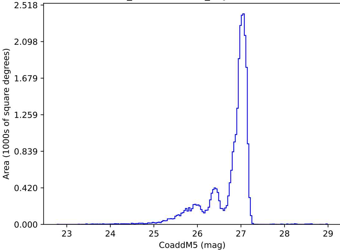
weather_cloudso14v3.4_10yrs r: CoaddM5
