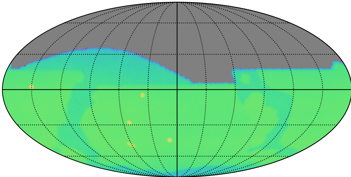
weather_cloudso14v3.4_10yrs : CoaddM5
