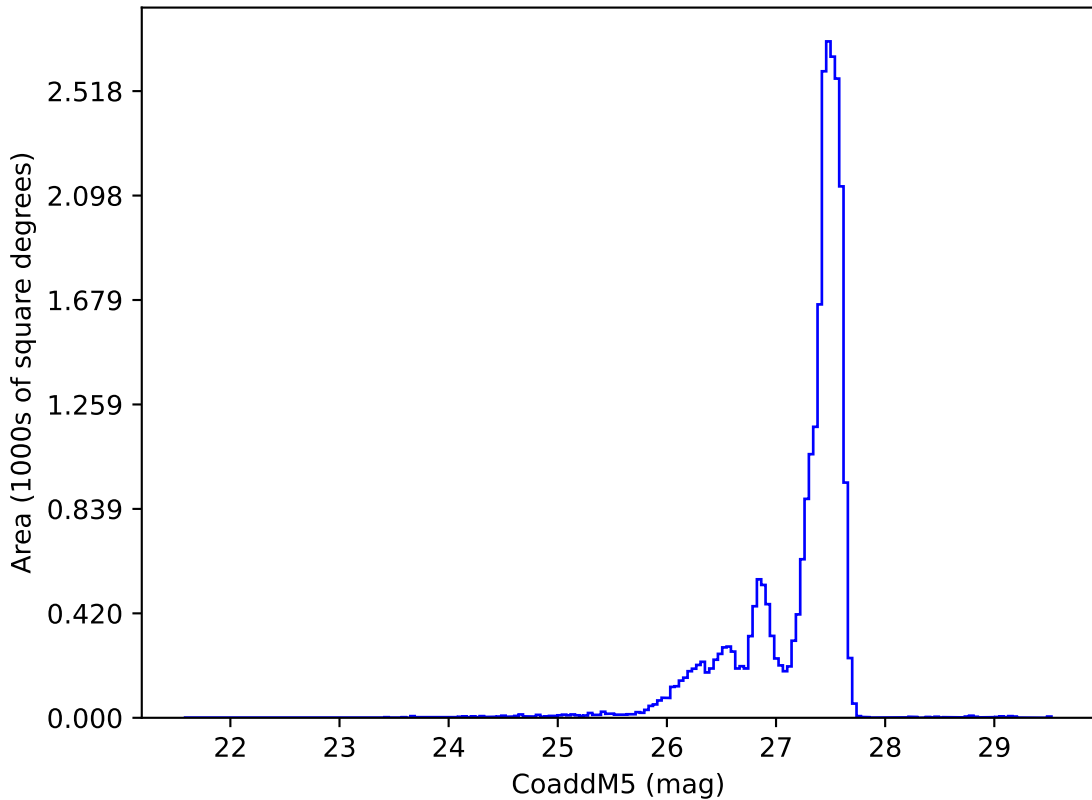
weather_cloudso14v3.4_10yrs : CoaddM5
