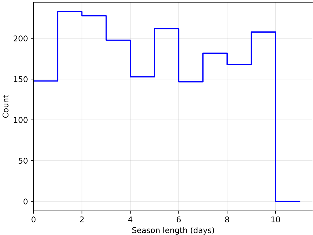
weather_cloudso14v3.4_10yrs DD:WFD all bands: SeasonLength
