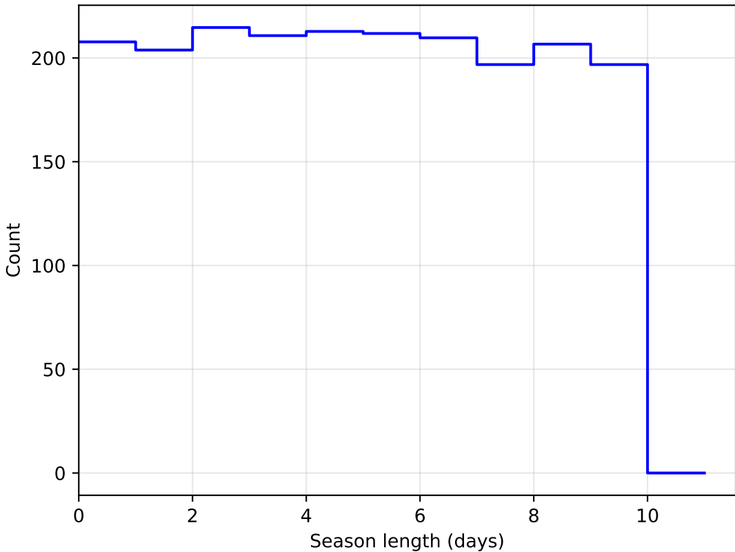
weather_cloudso14v3.4_10yrs DD:EDFS all bands: SeasonLength
