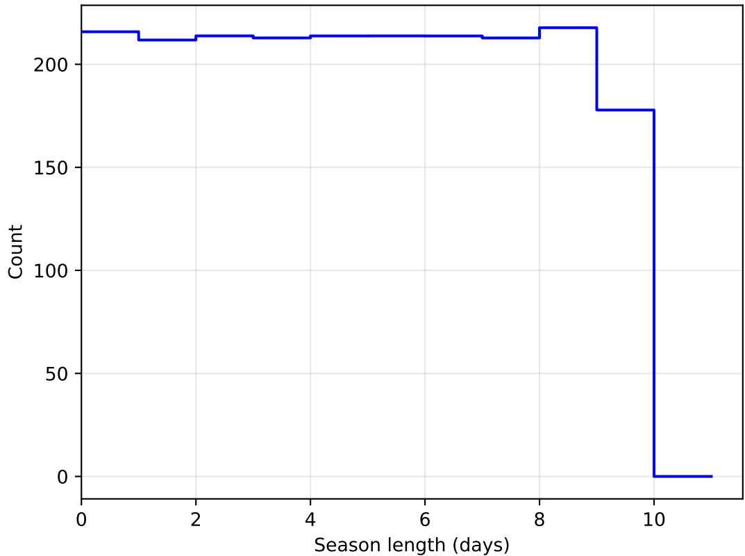
weather_cloudso14v3.4_10yrs DD:ECDFS all bands: SeasonLength
