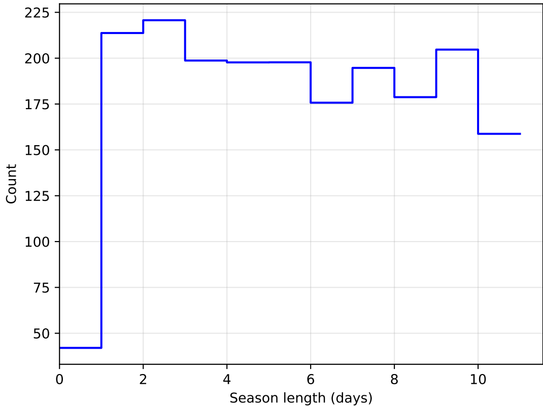
weather_cloudso14v3.4_10yrs DD: COSMOS all bands: SeasonLength
