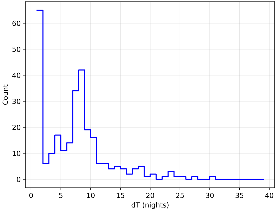
weather_cloudso14v3.4_10yrs all bands: DD:XMM_LSS Delta Nights Histogram
