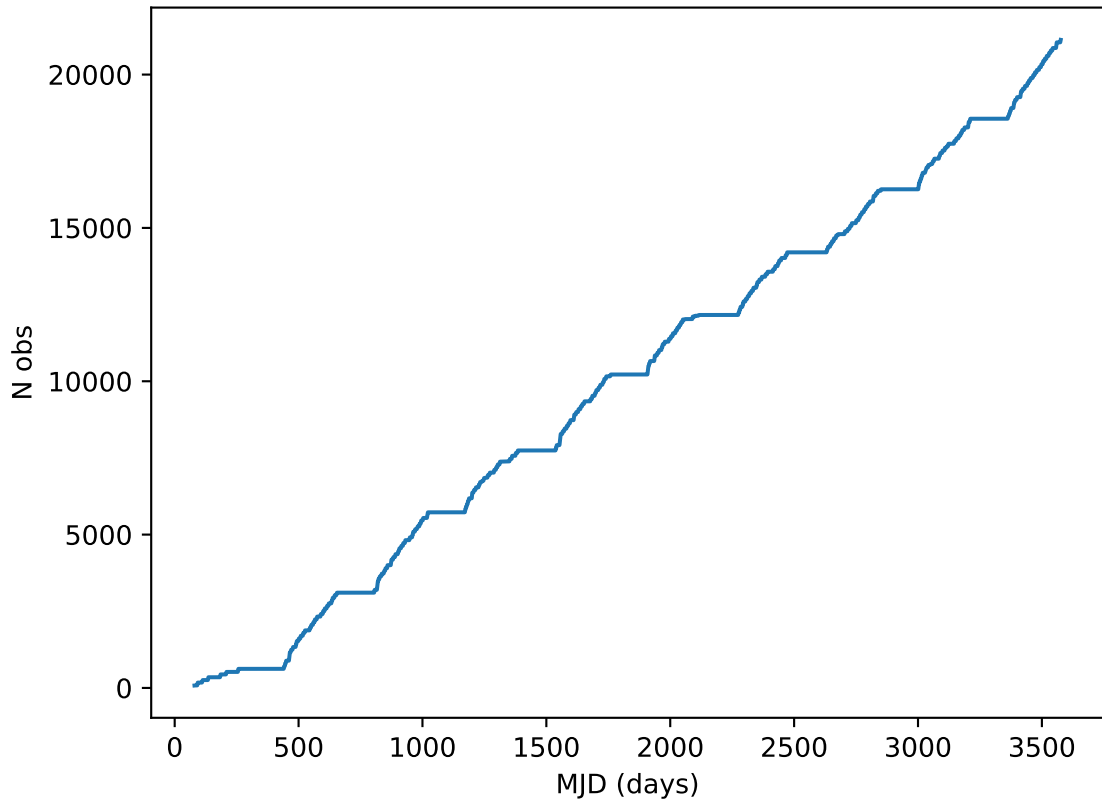
weather_cloudso14v3.4_10yrs all bands: DD:XMM_LSS Cumulative NVisits
