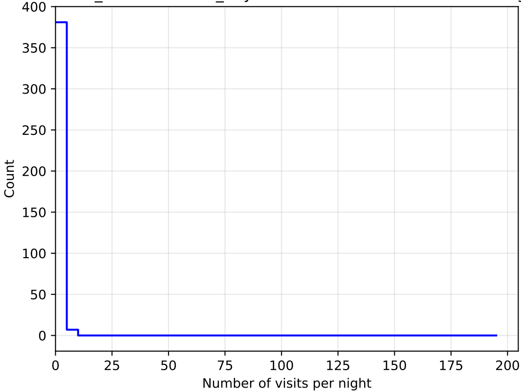
weather_cloudso14v3.4_10yrs all bands: DD:WFD NVisitsPerNight
