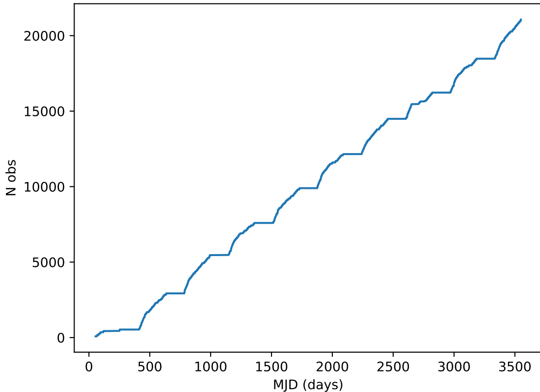
weather_cloudso14v3.4_10yrs all bands: DD:ELAISS1 Cumulative NVisits
